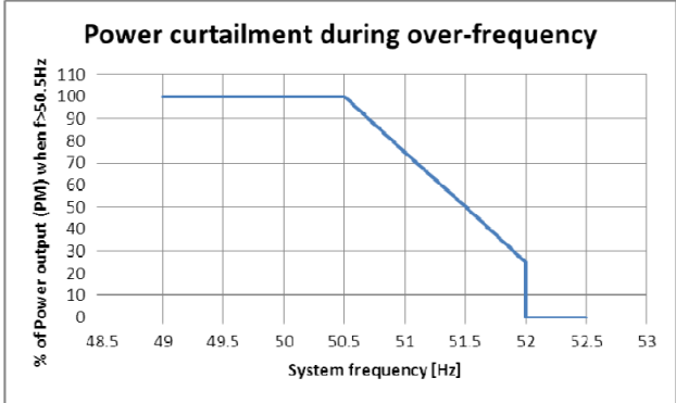
Figure 5 — Power curtailment during over-frequency
