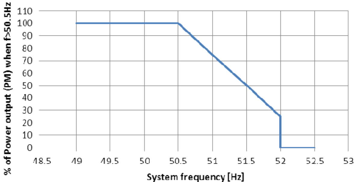
Power curtailment during over-frequency
